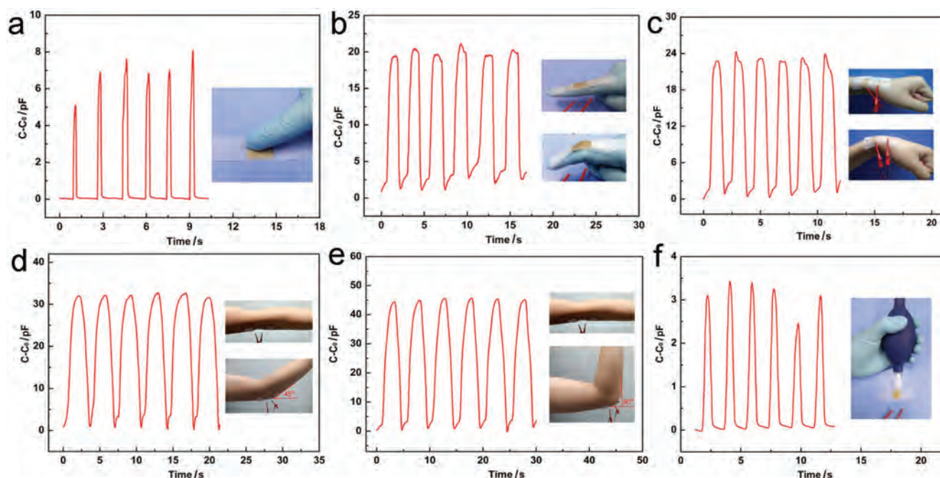
Figure 5. Real-time monitoring of capacitance changes upon pressing caused by repeated a) finger touching, b) finger bending, c) wrist bending, d,e) elbow bending with a 45° and a 90° angles, respectively, and f) airflow.
